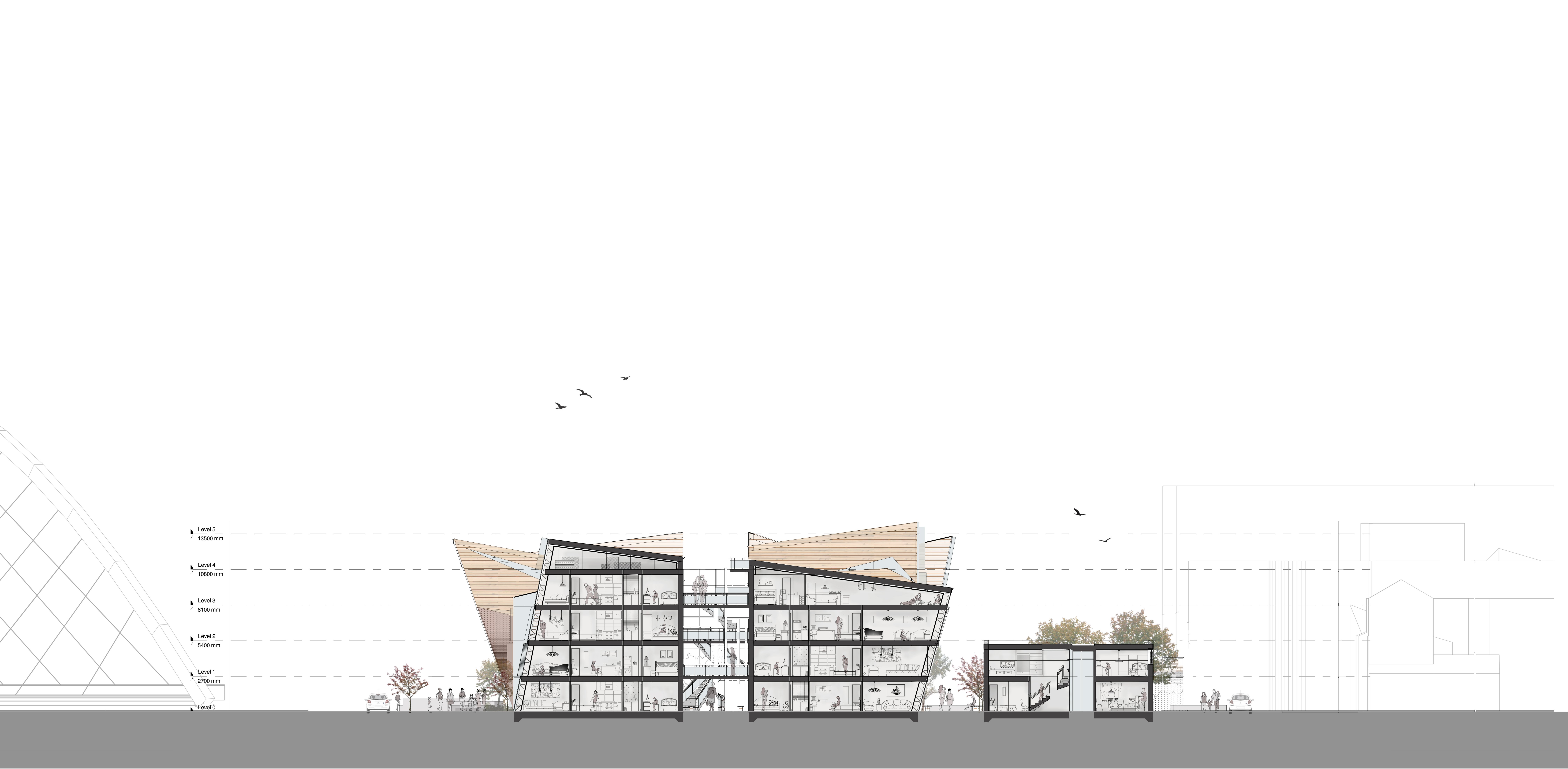
1 Cross section- south facing 1 : 100
