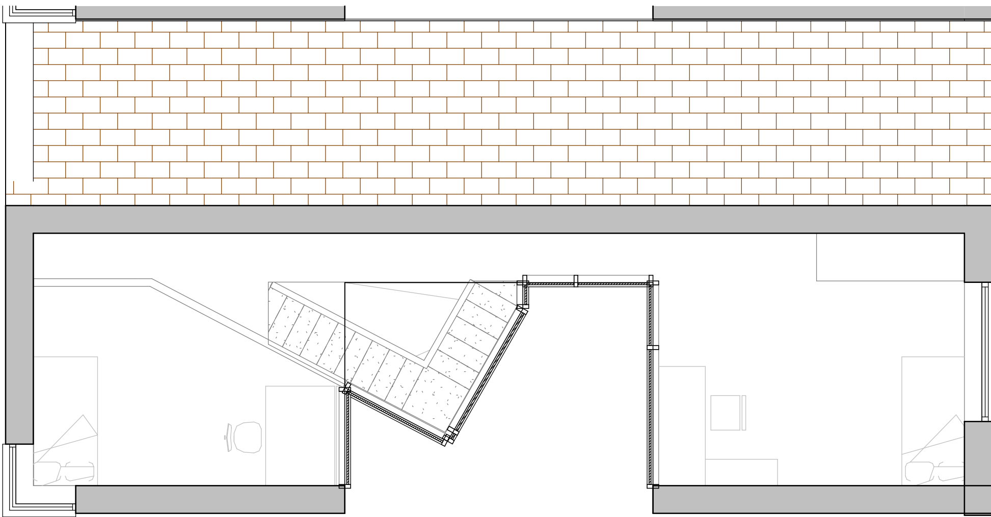
1 Housing unit - type A (first storey) 1 : 50
